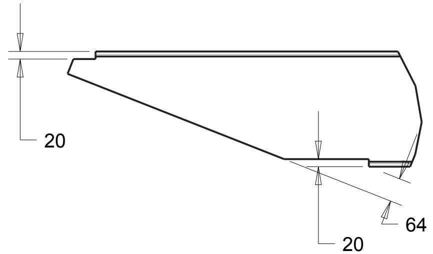
DETAIL A-ALT SCALE 0.100 ALTERNATE MANUFACTURING METHOD REMOVE MATERIAL AS SHOWN
